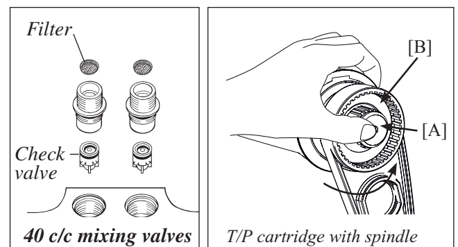
Dismounting and attaching the T/P cartridge head piece.
